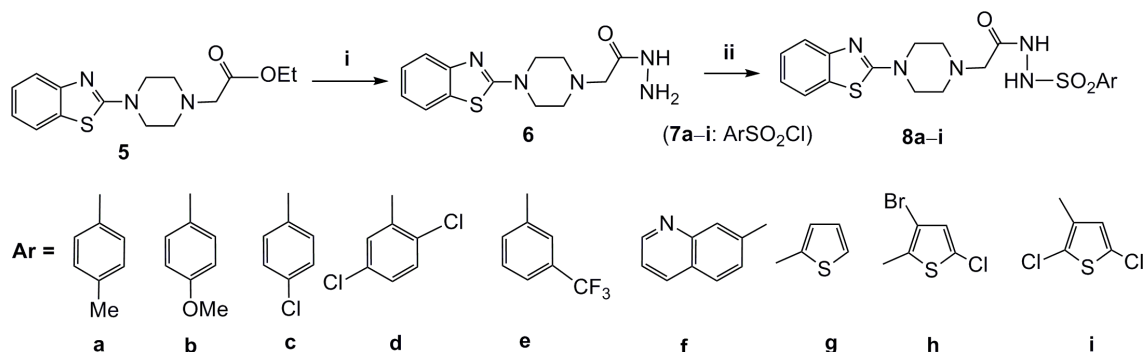
Scheme 2. Reagents and conditions: i) EtOH, \text{NH}_2\text{NH}_2 \cdot \text{H}_2\text{O} , reflux, 8 h; ii) \text{CHCl}_3 , 7a–i , \text{Et}_3\text{N} , r. t., 20–24 h.
